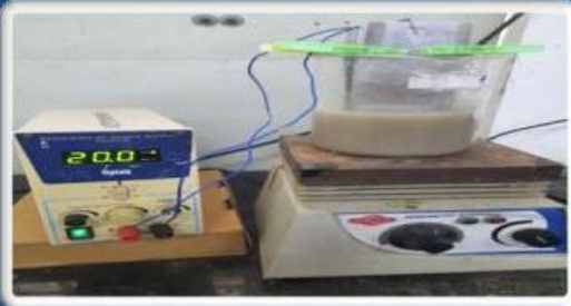
Removal of fluoride from water by electrocoagulation process
